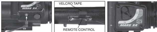
FIGURE 2-9 . REMOTE CONTROL
