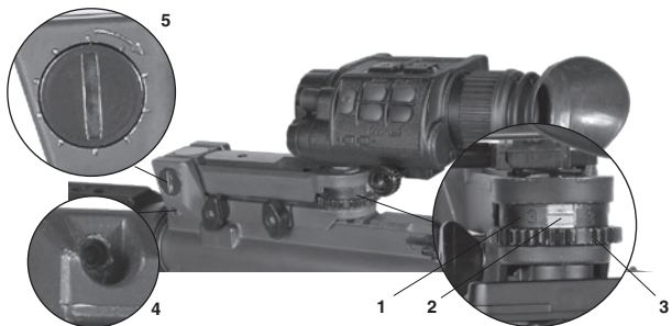
Figure 3-7. Windage and Elevation Adjustment
