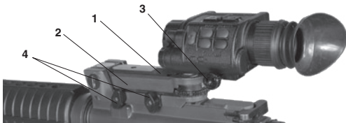
Figure 2-8. Weapon Mount
