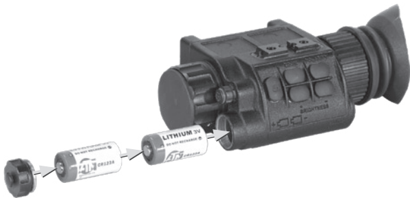
Figure 2-1. Install batteries
